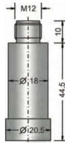
2-wire, 4...20mA
