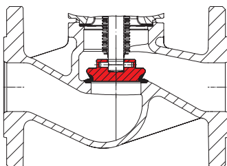
Isolation plug with marginal seat
